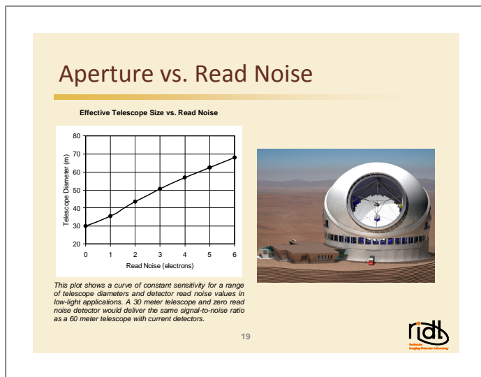
Figure 1: Read noise versus effective aperture
